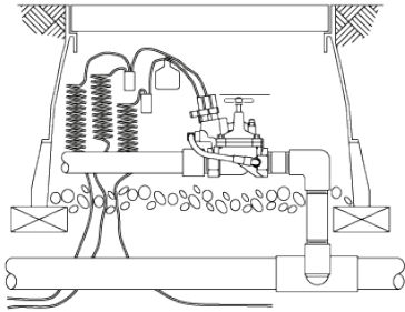
Brass Electric Remote Control EFB-CP Valve
